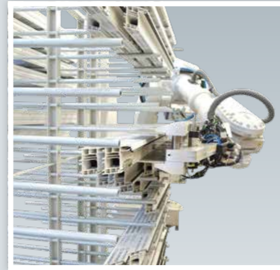
Greiferzange in Ablageposition gripper in rest position
