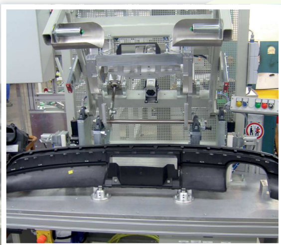
Handklebevorrichtung Abdeckung Anhängerkupplung manual gluing cell for trailer coupling cover
